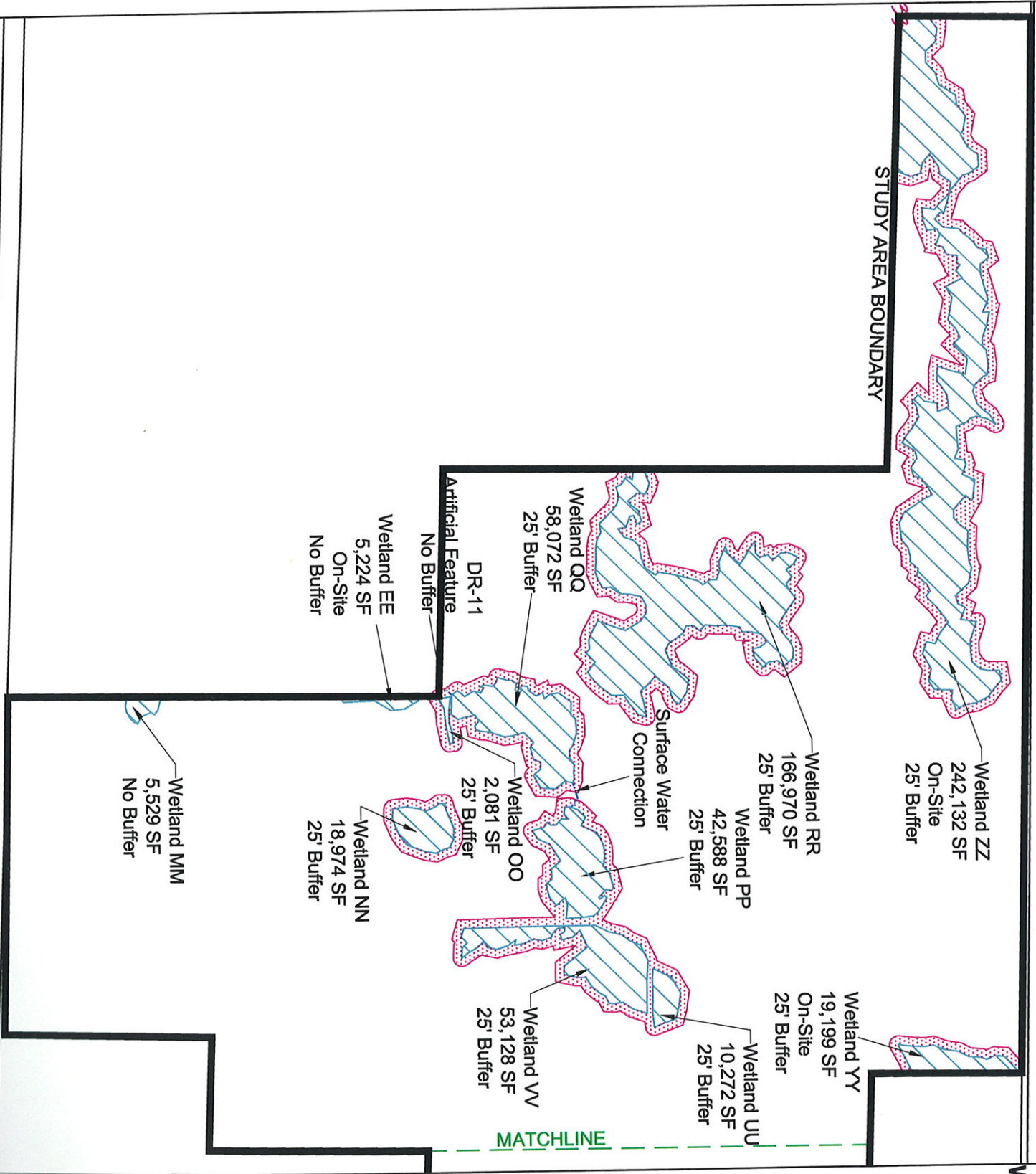
Figure 10. Wetland Delineation Map West Portion Grandis Pond October 18, 2006
